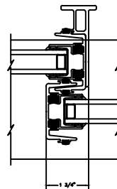
5 MEETING STILE PB200
