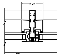
7 VERTICAL TRUE MUNTIN PB200
