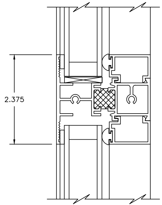
② TRUE MUNTIN FIXED
