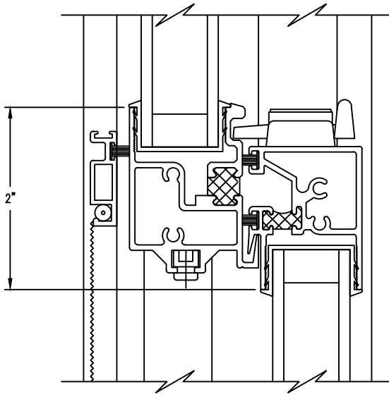
② MEETING RAIL DOUBLE HUNG
