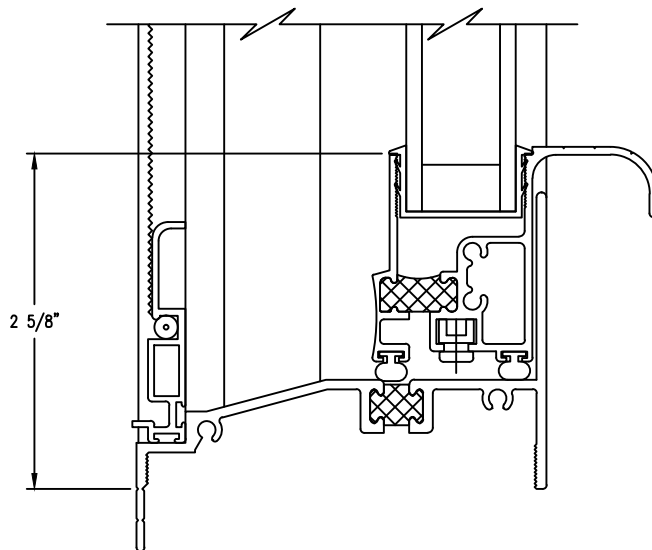
③ SILL DOUBLE HUNG
