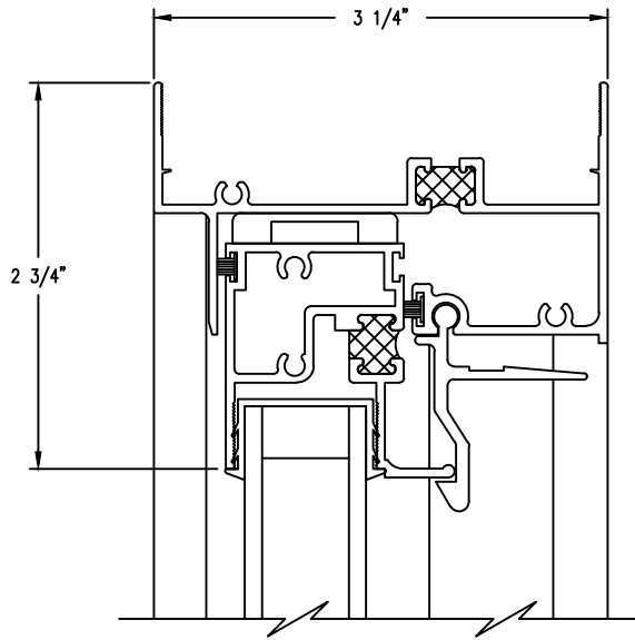
① HEAD DOUBLE HUNG
