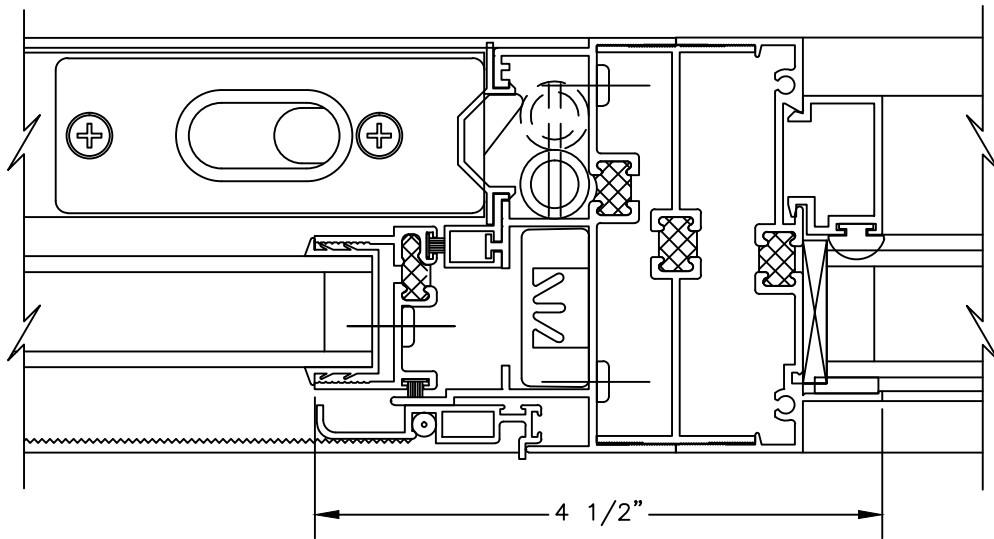
⑥ VERTICAL STACK MULLION DOUBLE HUNG/FIXED LITE
