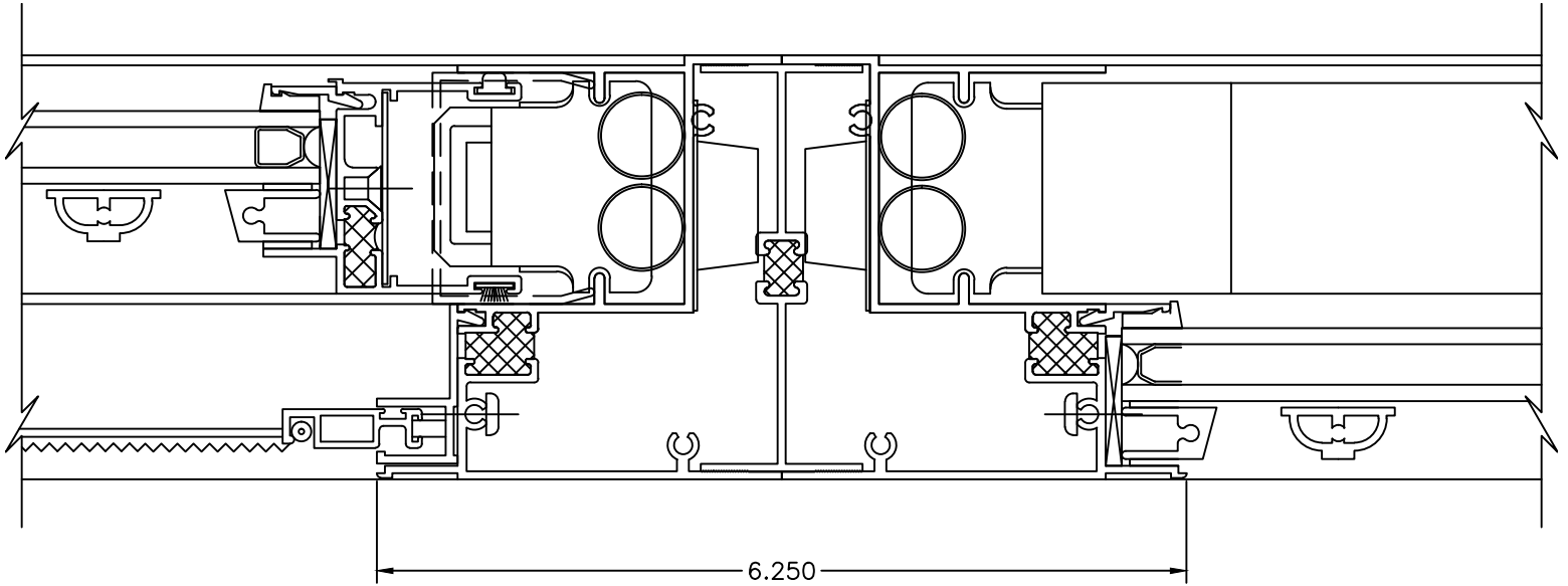
⑤ VERTICAL STACKING MULLION
