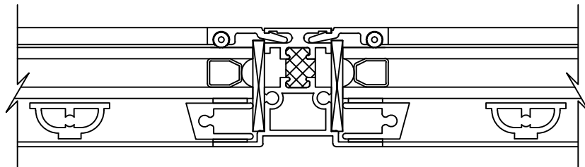
⑦ VERTICAL TRUE MUNTIN
