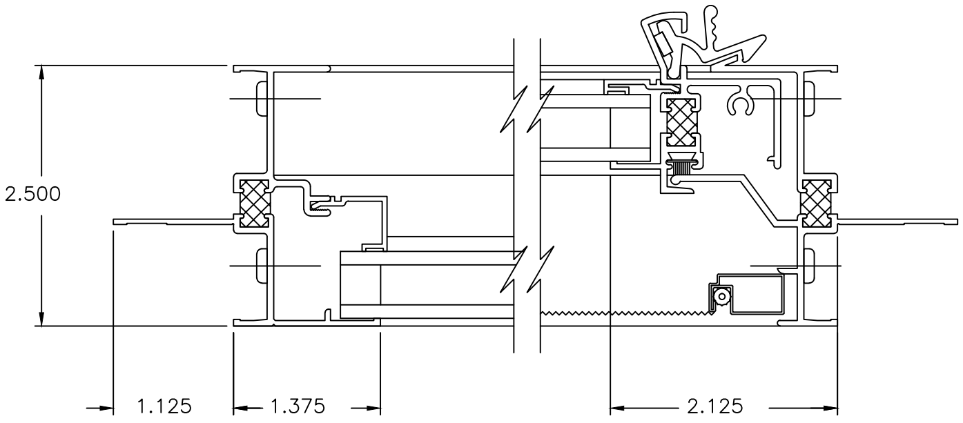
③ FIXED LEFT JAMB P5400 SINGLE SLIDE
