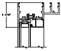
1 FIXED HEAD P6100
