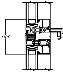
11 CASEMENT HORIZ INT MULLION P6100
