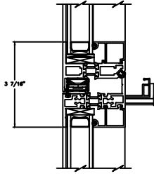
12 CASEMENT HORIZ INT MULLION P6100
