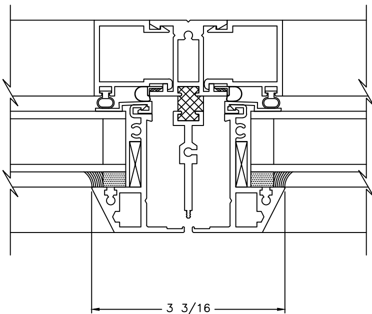
⑤ INTEGRAL MULLION P7500
